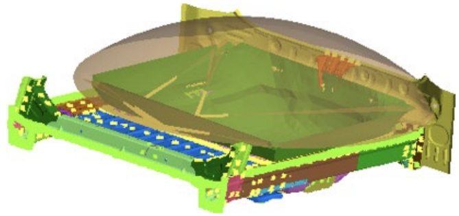
Figure 2: Lightweight hybrid tub
