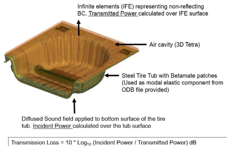
Figure 3: Spare tire tub Dura Lightweight Hybrid Design
