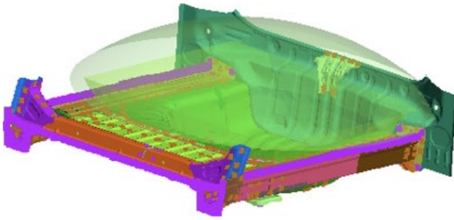
Figure 1: Spare tire tub base design
